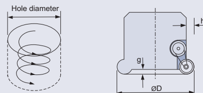
Helical milling
